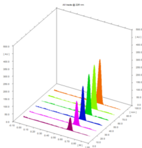
Fig. 2: Linearity of PMT
